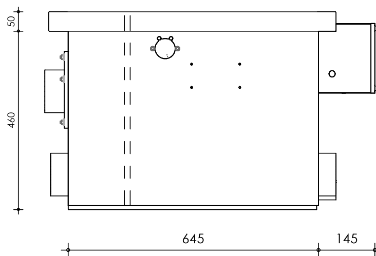
Right-side view
