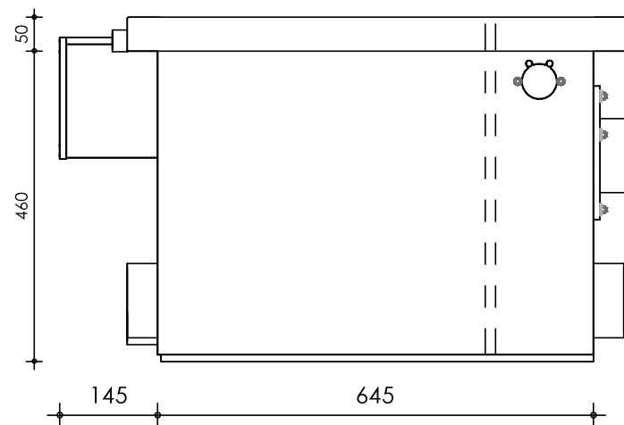
Left-side view
