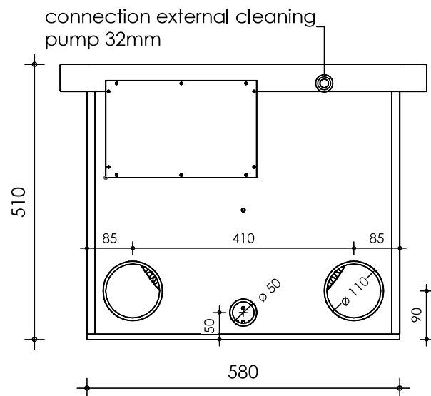
Rear view
