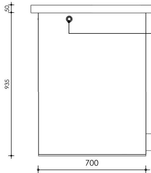
Left-side view
