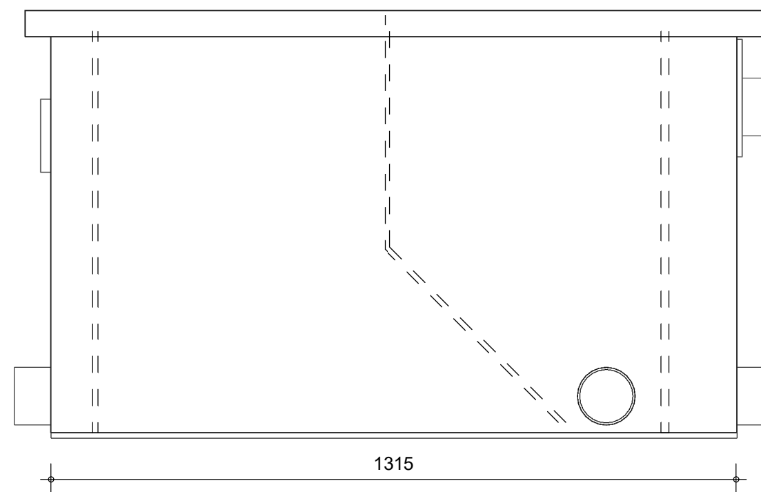
Left-side view
