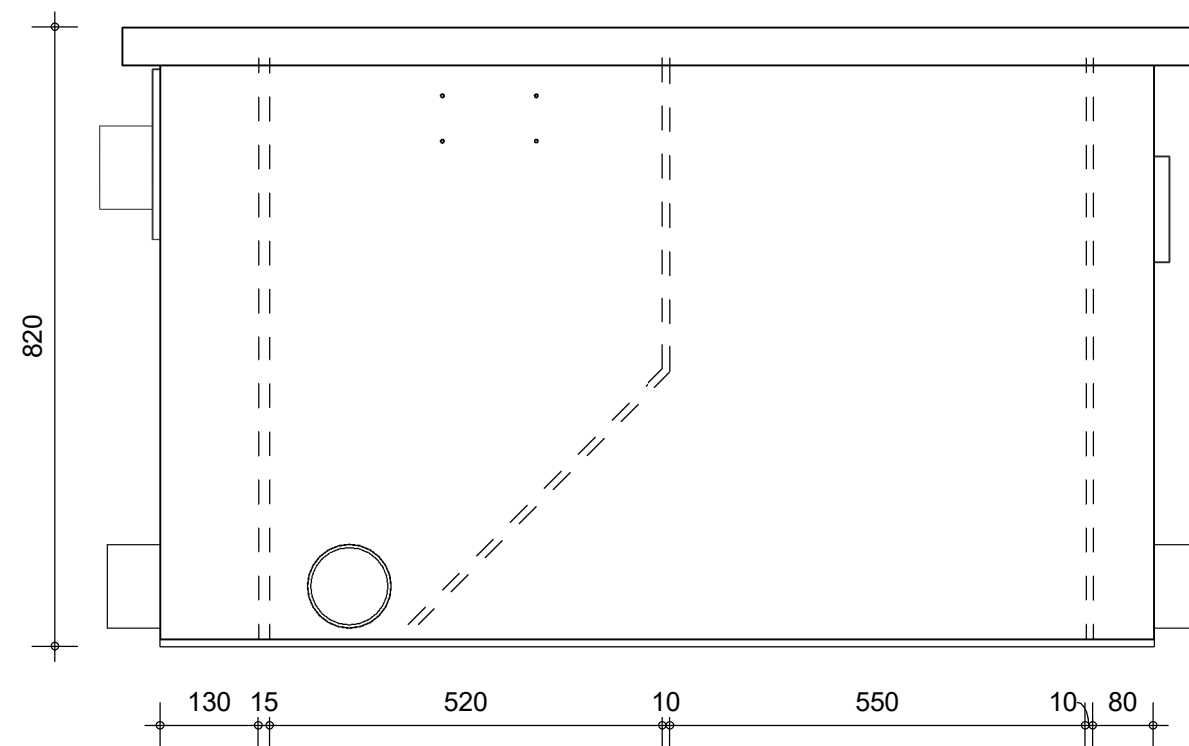
Right-side view
